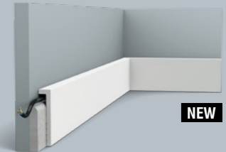
SX171 SQUARE SX171-RAL9003 200 x 10 x 2,2 cm Duropolymer®
