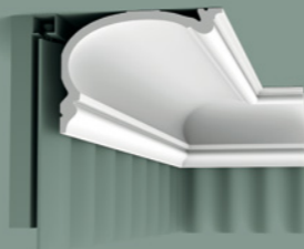
C342 HERITAGE CURTAIN PROFILE 200 x 14 x 19 cm Purotouch®
